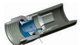
Compact ferrule
